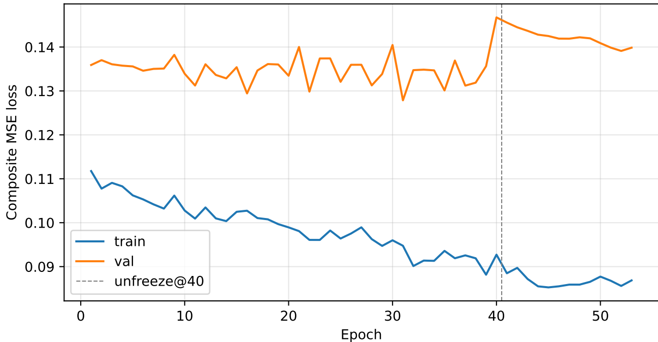
Training curves - warfarin
