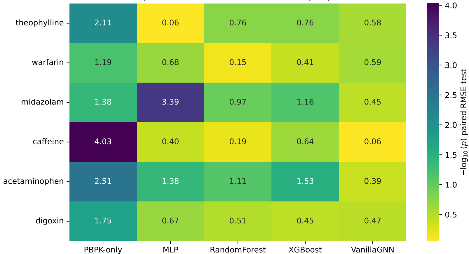
Phase 2.3 — paired t-test: baseline vs DL-PBPK (per-patient RMSE)
