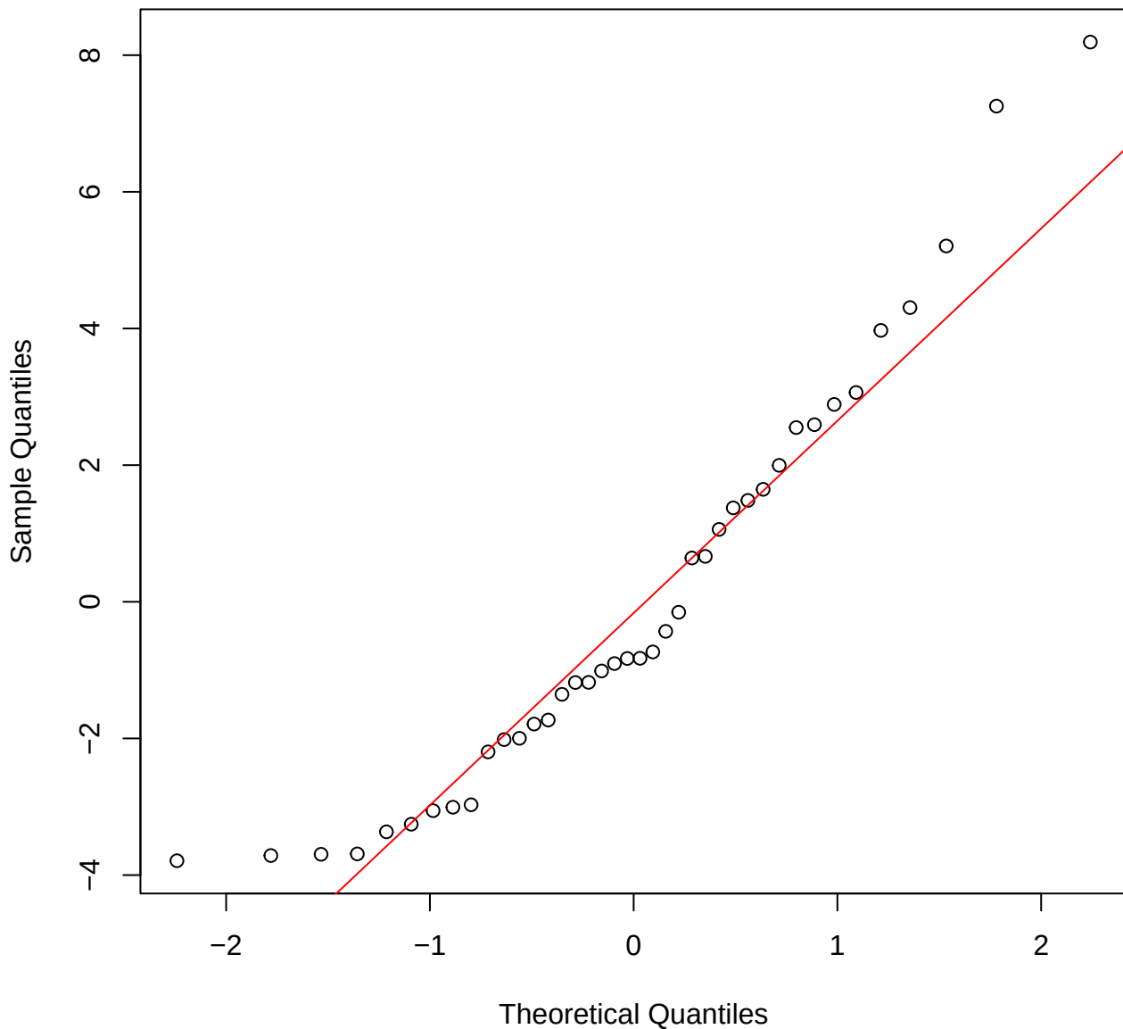
QQ plot residuals – Roots
