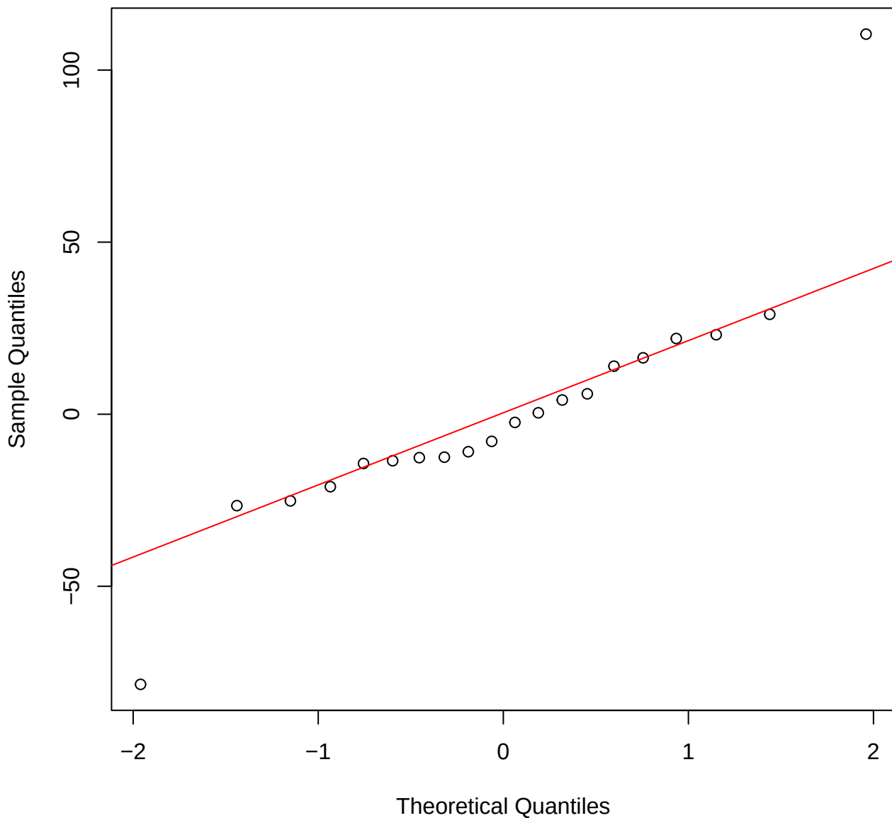
QQ plot residuals – Rhizo
