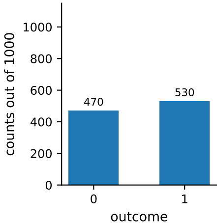
Z basis
