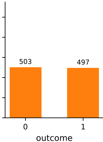
X basis
