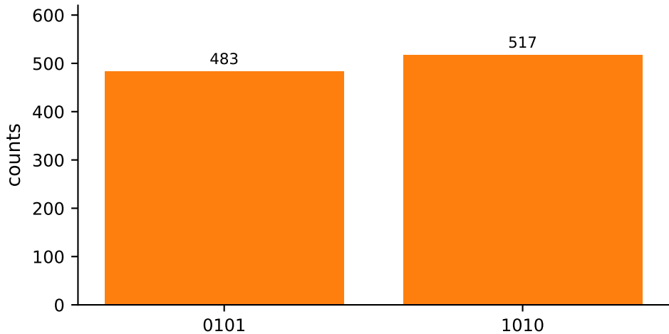
samples of the optimized QAOA state, p = 2
