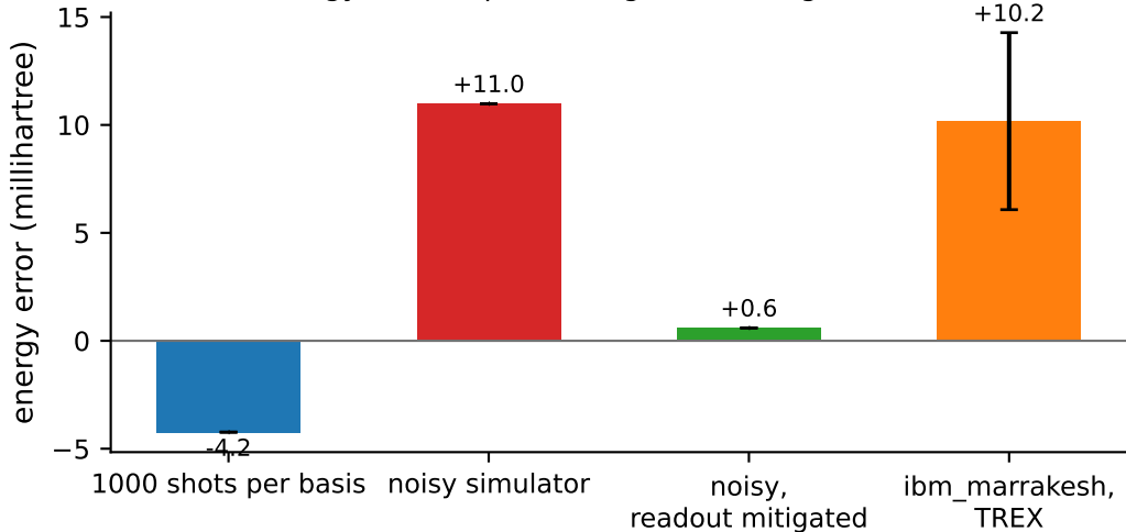
energy at the optimal angles, error against exact
