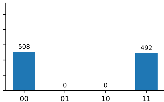
|+\rangle|+\rangle , XX basis
