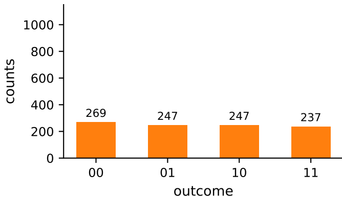
|+\rangle|+\rangle , ZZ basis
