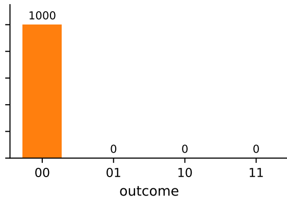
|+\rangle|+\rangle , XX basis
