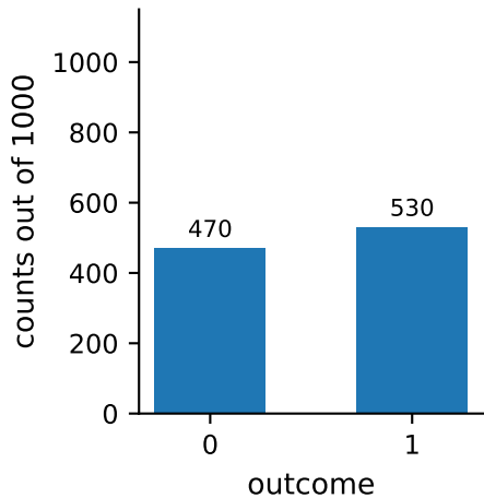
Z basis
