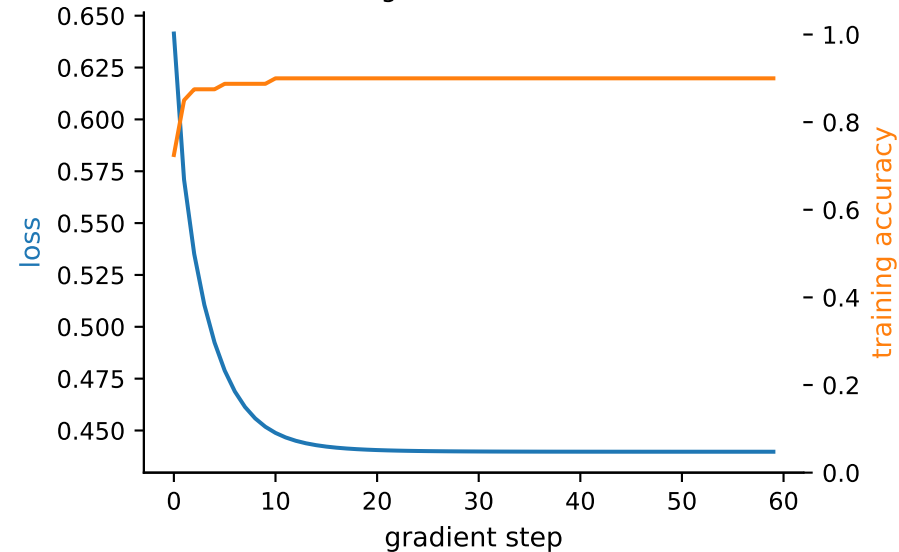
training on the circles data
