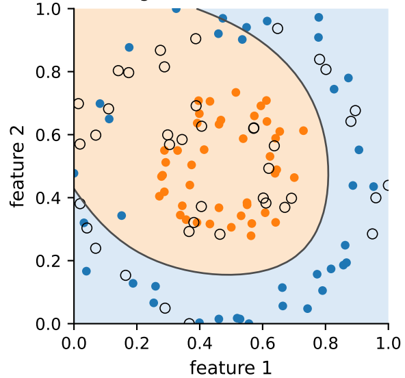
sign of f(x; \theta) , test 78%
