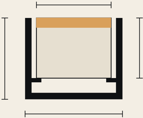
STRIP 16.5 × 16.5MM — CHANNEL OR-AL-CC 20.4 × 19.6MM SECTION VIEW, TO SCALE. EMITTING FACE UP.
