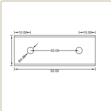
HOLE LAYOUT
