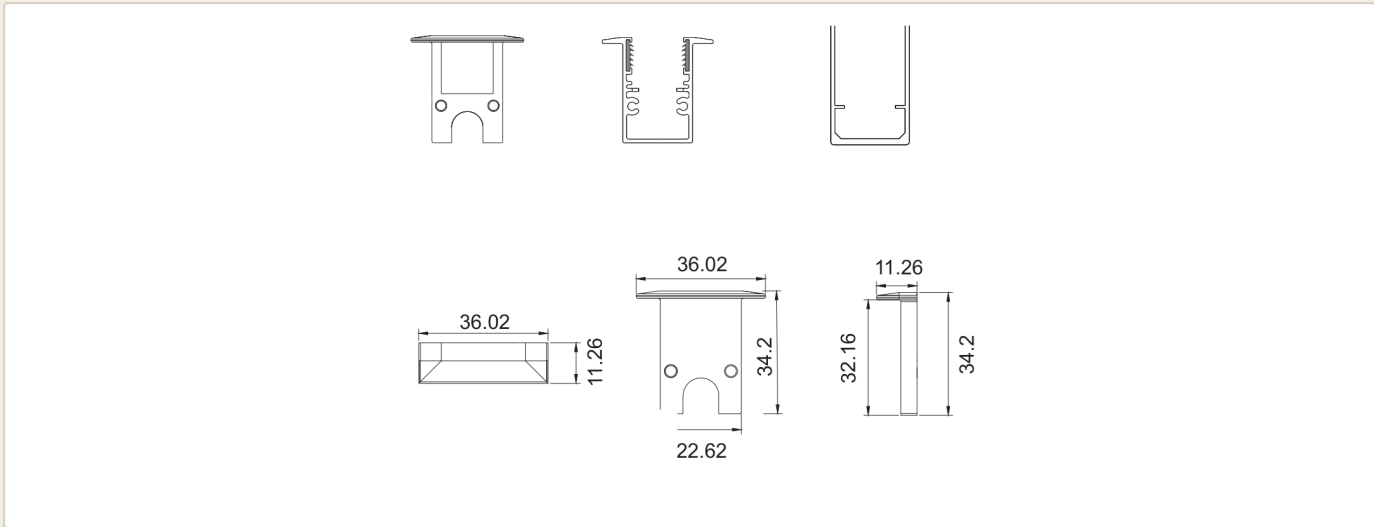
PROFILE SECTIONS — MM
