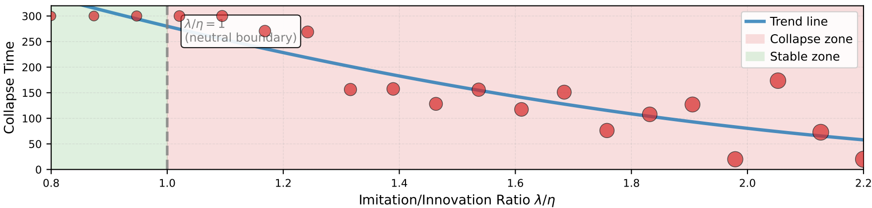
(E) Collapse Time vs \lambda/\eta Ratio
