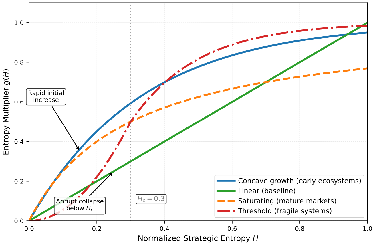
Figure 2: Four Canonical Entropy Multiplier Regimes
