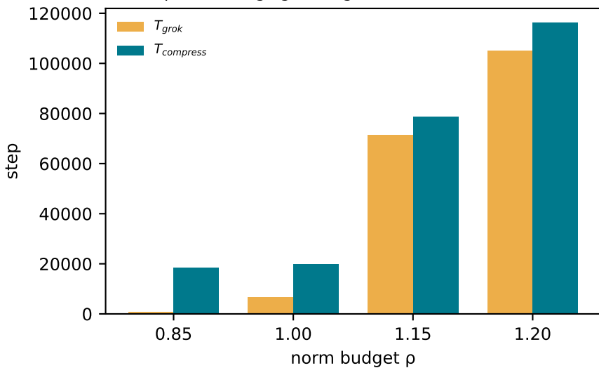
C compression lags grokking
