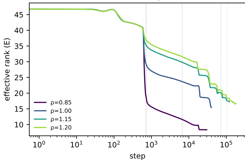
C compression lags grokking
