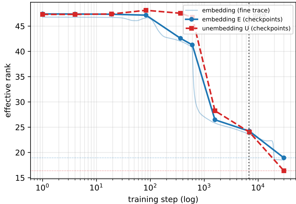
\rho = 1.00 (median acc = 0.994) both loci collapse around grok to a shared floor ( \approx 17.7 )
