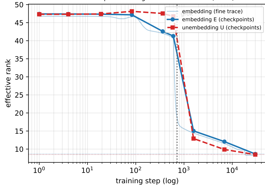
\rho = 0.85 (median acc = 1.000) both loci collapse around grok to a shared floor ( \approx 8.6 )
