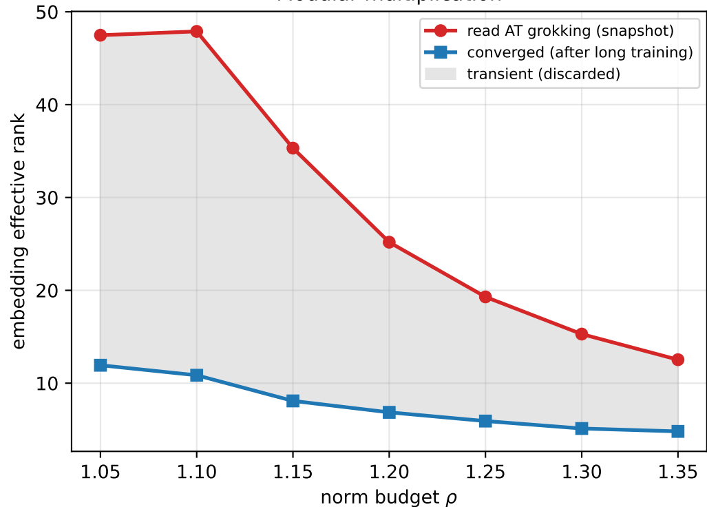
Modular multiplication
