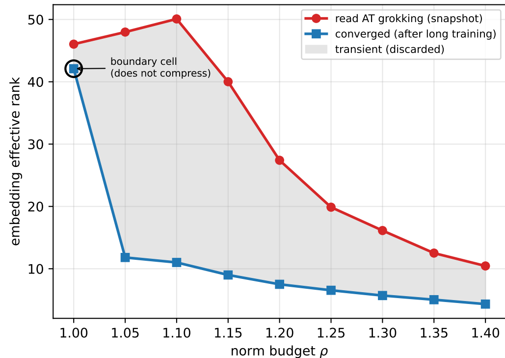
Modular addition
