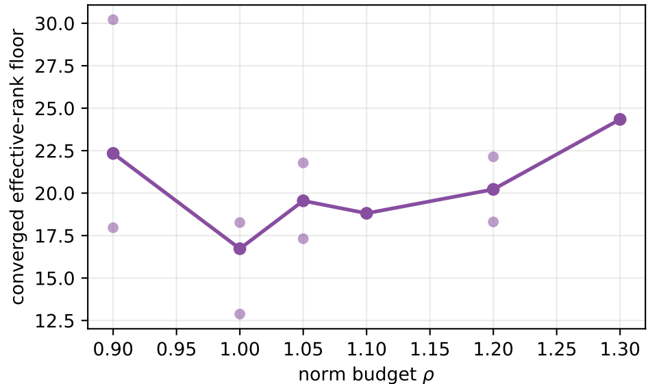
Transformer embedding (this work) Spearman( \rho , floor) = +0.14 ( p=0.66 ) — no depth law
