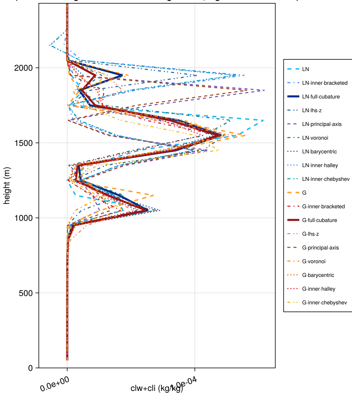
TRMM SGS smoke (N=4, z164_dt150s): clw + cli, final output time (cool hues = lognormal · warm hues = gaussian; legend lists LN then G)
