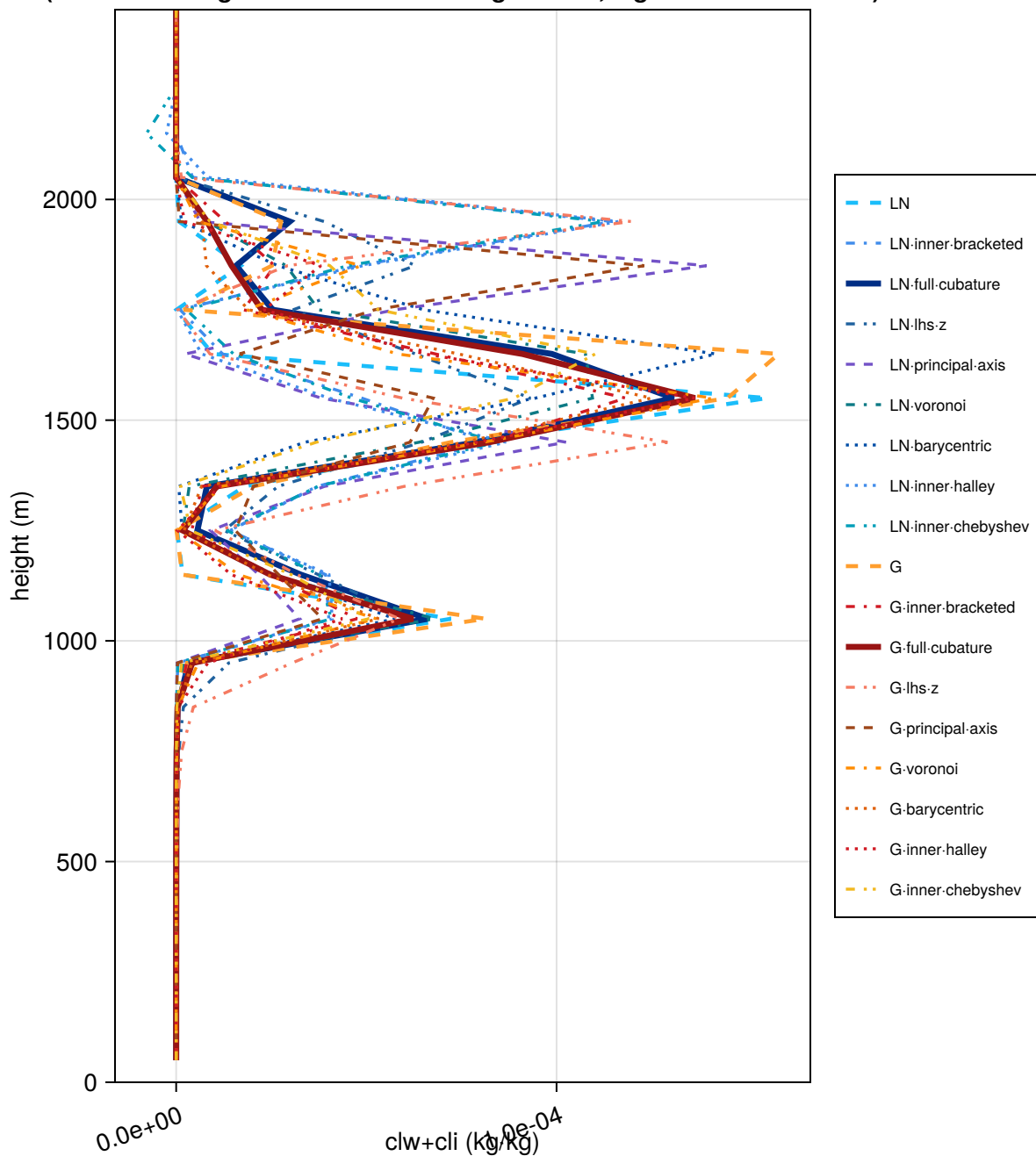
TRMM SGS smoke (N=5, z164_dt150s): clw + cli, final output time (cool hues = lognormal · warm hues = gaussian; legend lists LN then G)
