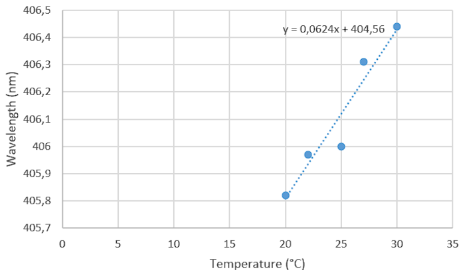
Figure 5: Temperature dependence of the pump laser wavelength (qualitative)
