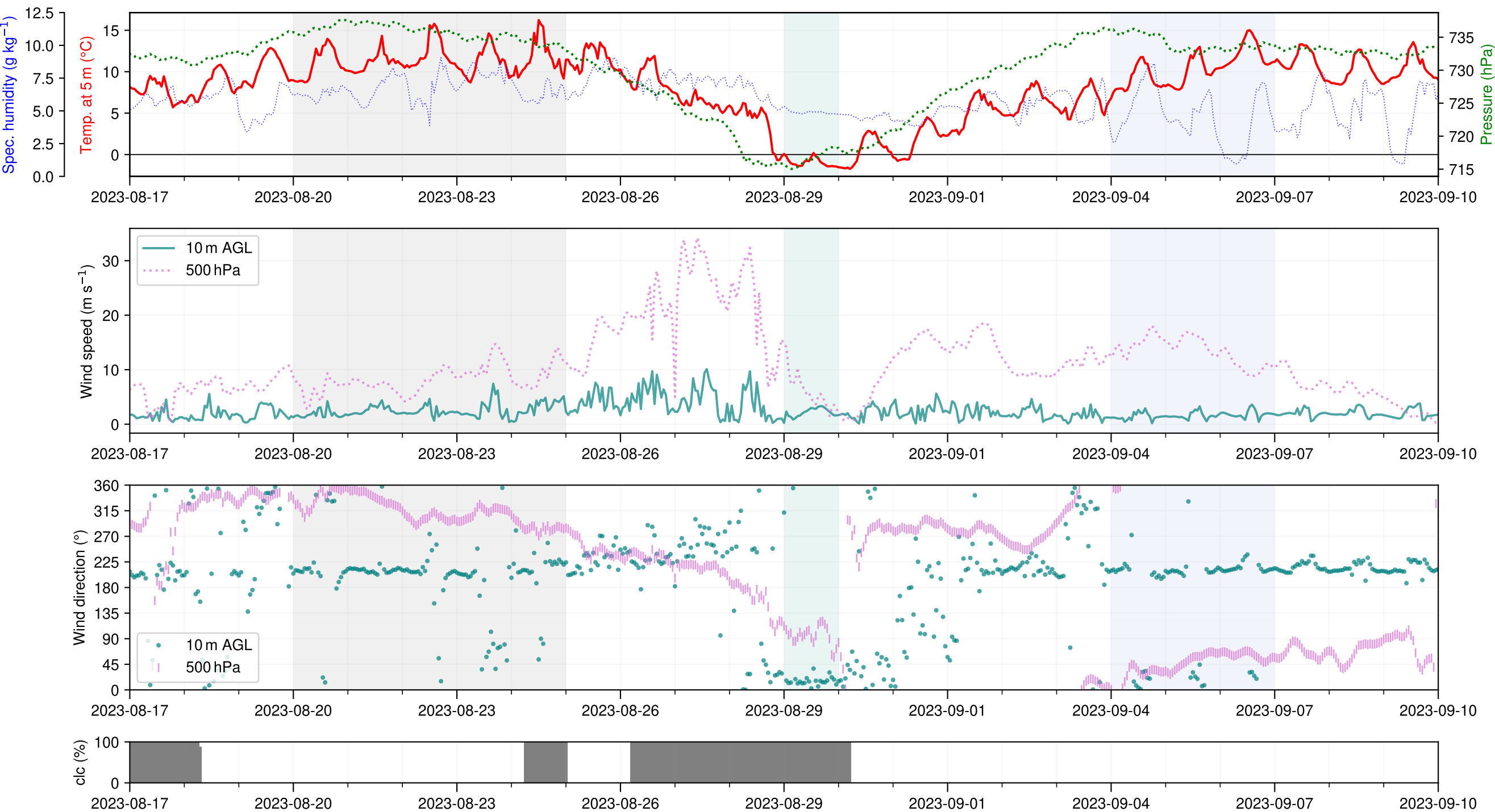
HEFEX II ICON output for grid cell 35714 (tower location)
