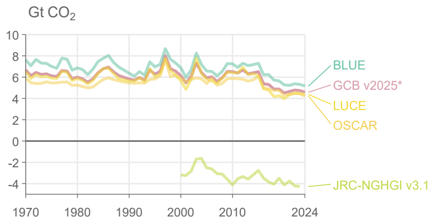
(c) Global CO 2 emissions from land use change (LULUCF)
