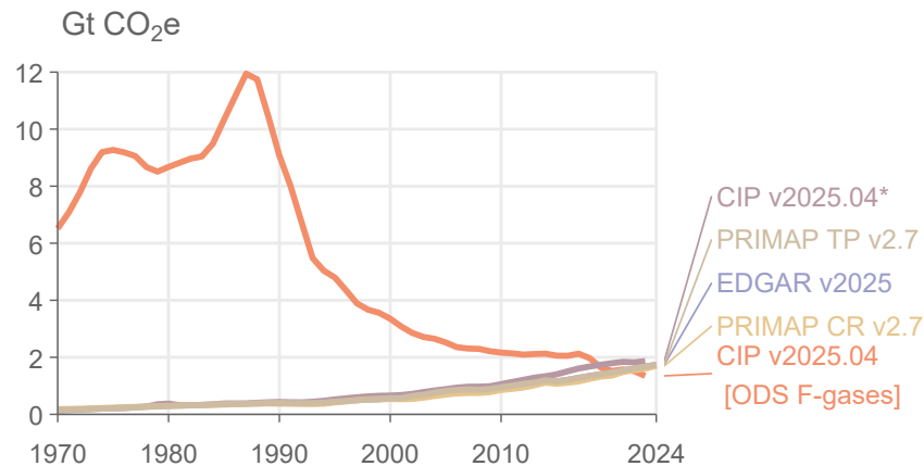
(f) Global F-gas emissions
