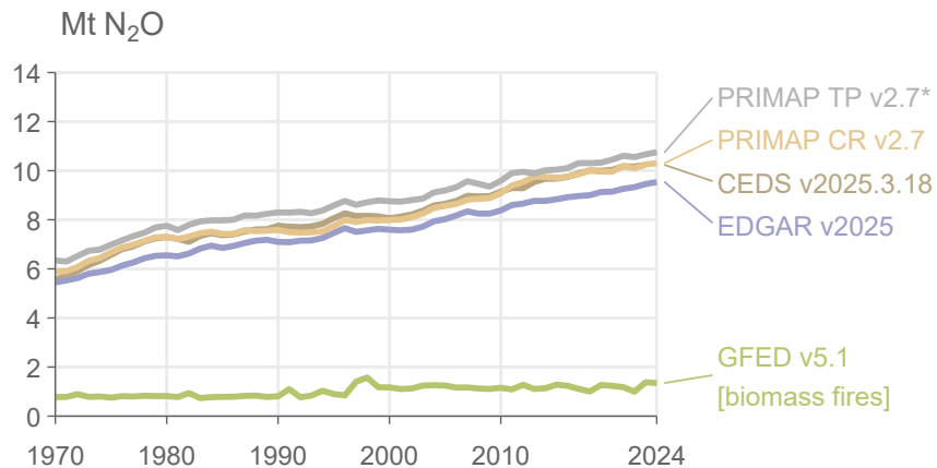
(e) Global N 2 O emissions
