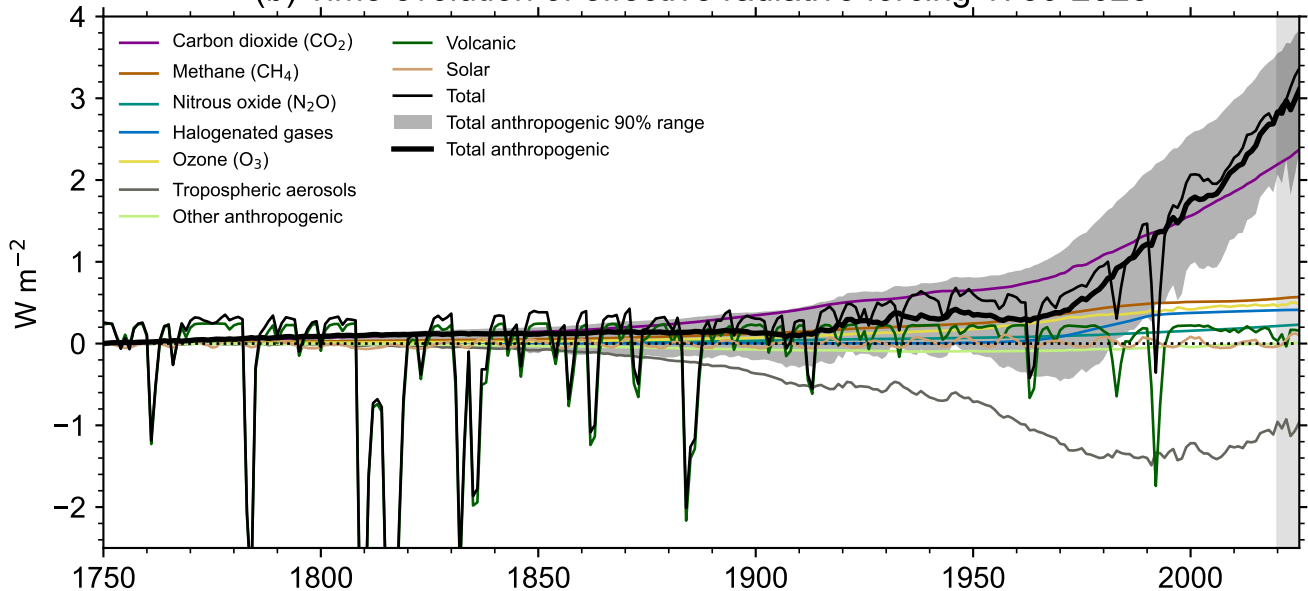
(b) Time evolution of effective radiative forcing 1750-2025
