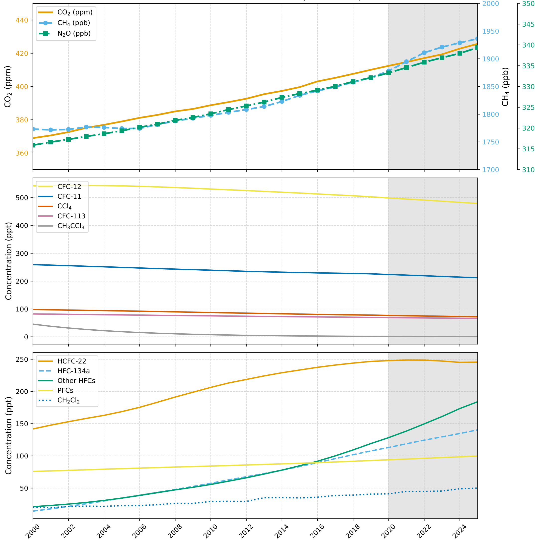
Greenhouse Gas Concentrations (2000-2025)
