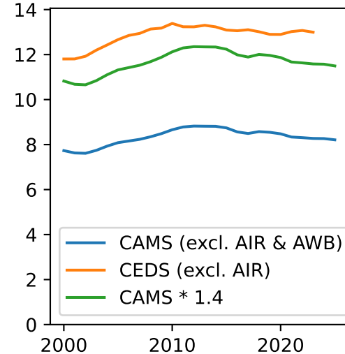
NH 3
