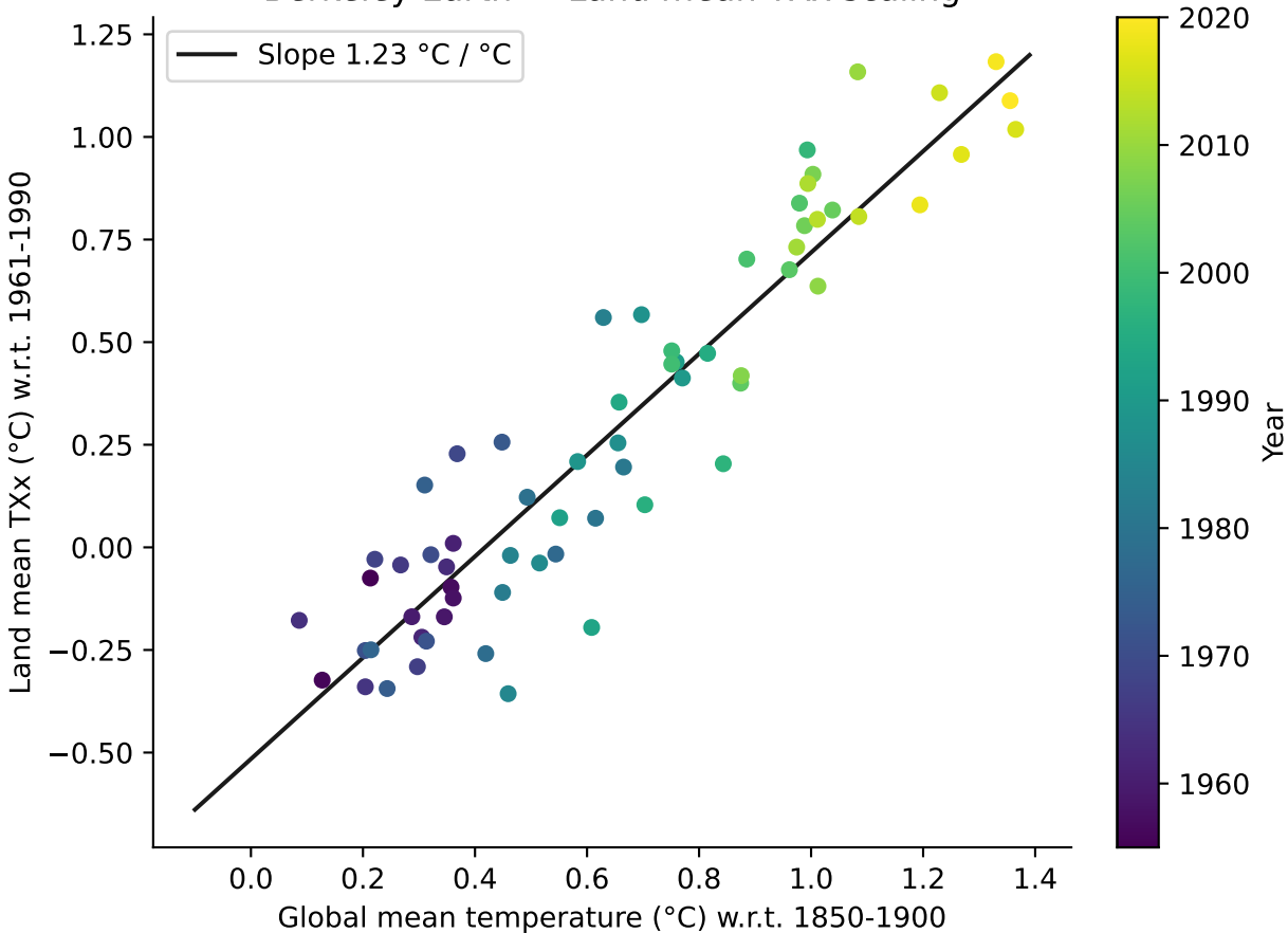
Berkeley Earth — Land mean TXx scaling
