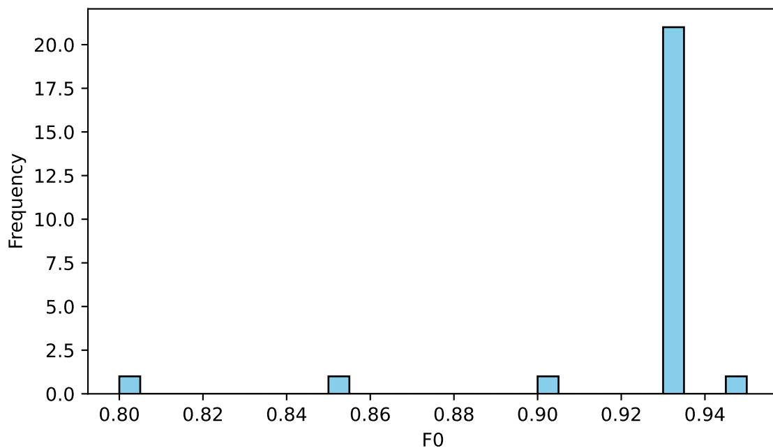
NLO Distribution
