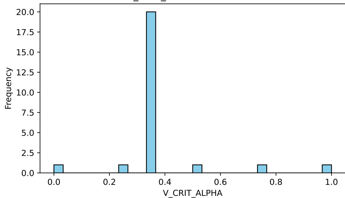
V_CRIT_ALPHA Distribution
