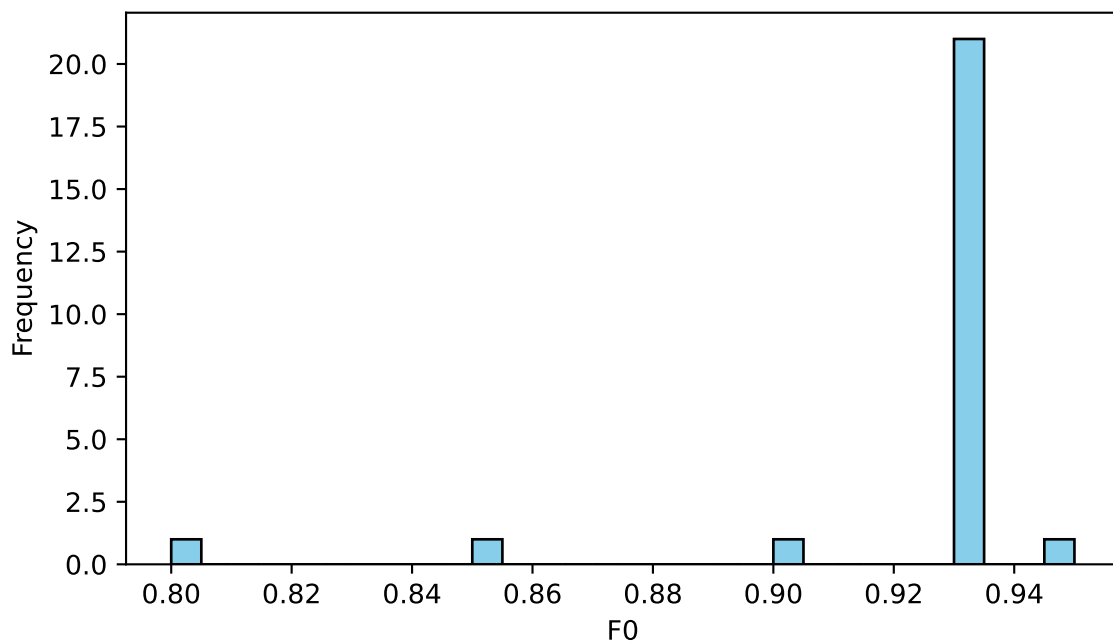
NLO Distribution
