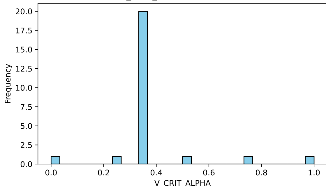
V_CRIT_ALPHA Distribution
