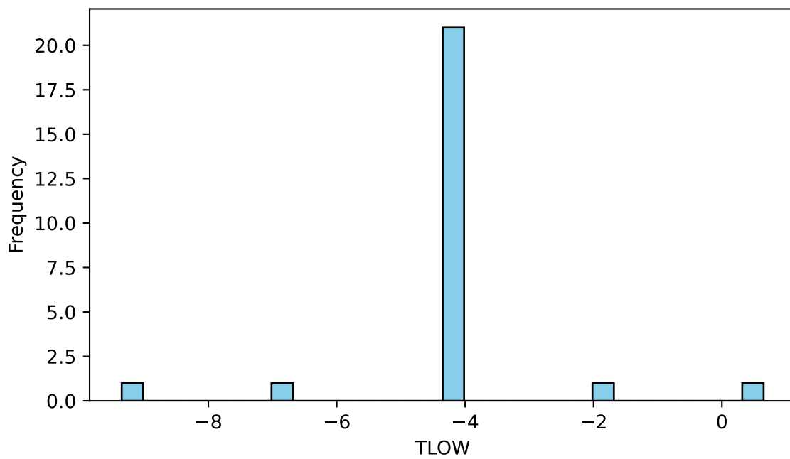
TLOW Distribution
