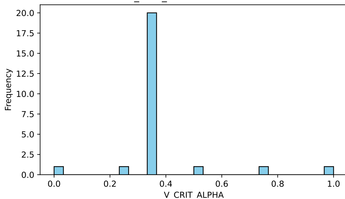
V_CRIT_ALPHA Distribution
