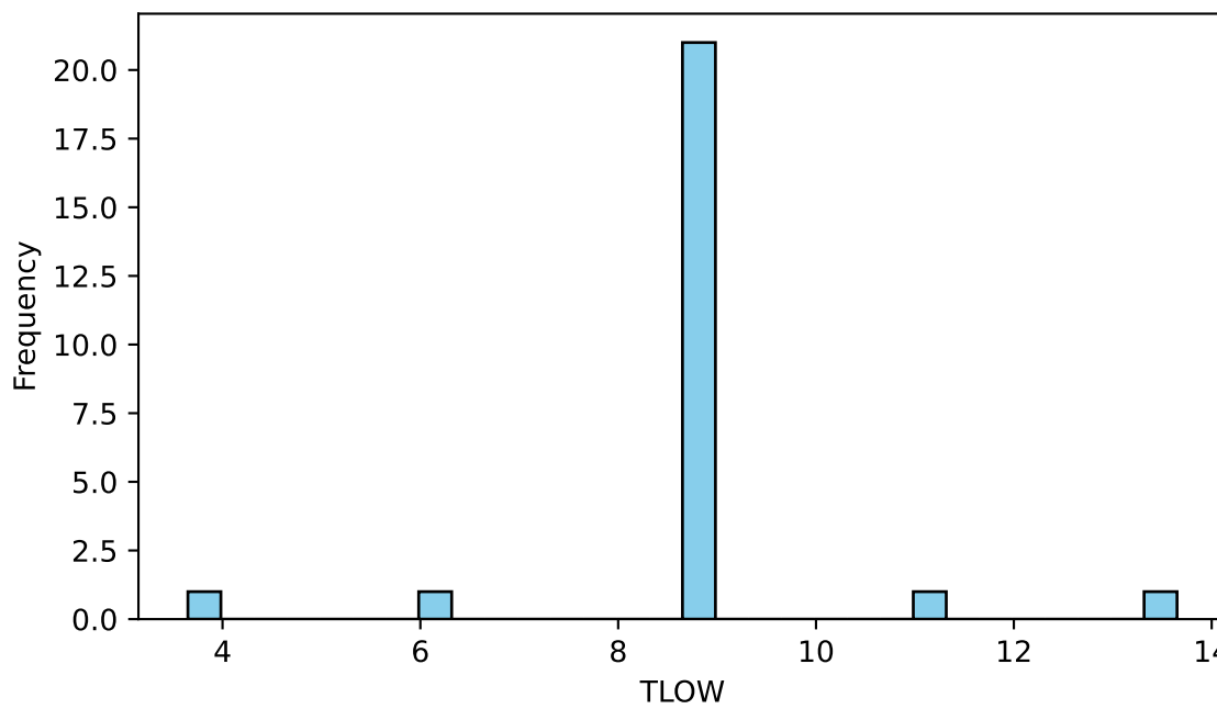
TLOW Distribution
