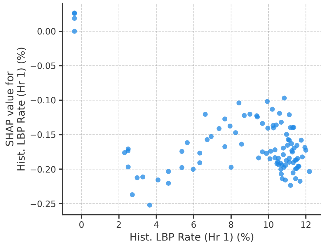
Fig 3B: SHAP Dependence (Hist. LBP Rate (Hr 1) (%))
