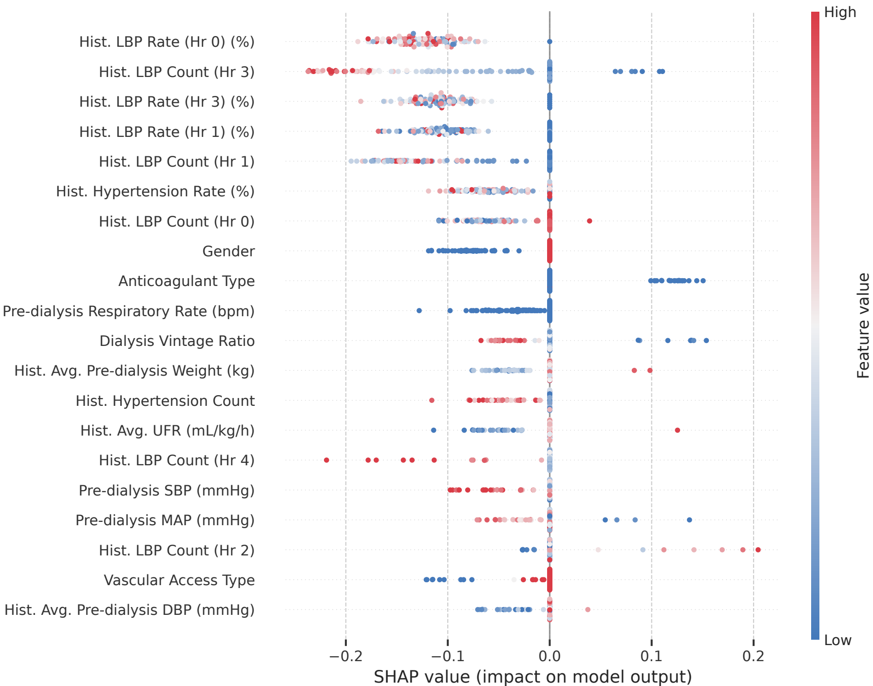
Fig 3A: SHAP Summary (Global Risk Drivers)
