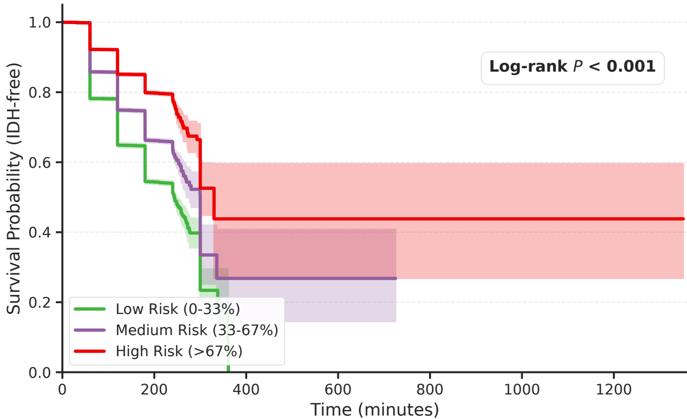
Fig 4: Kaplan-Meier Risk Stratification
