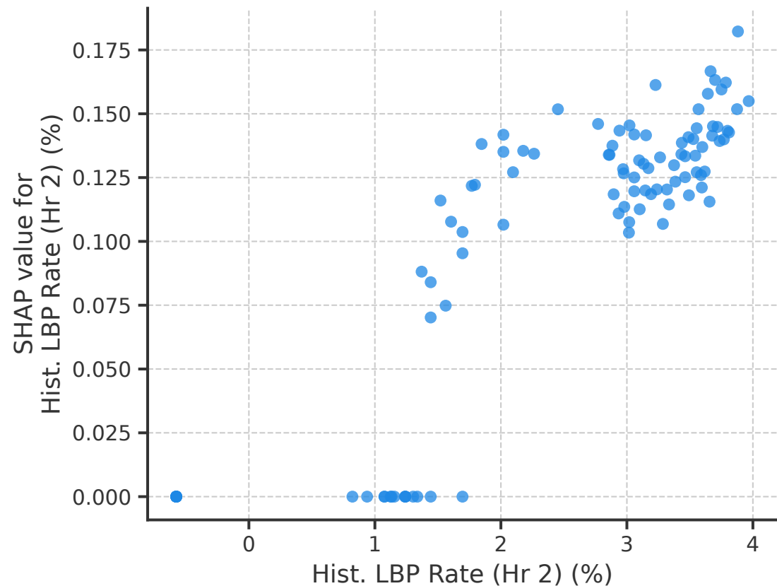
Fig 3B: SHAP Dependence (Hist. LBP Rate (Hr 2) (%))
