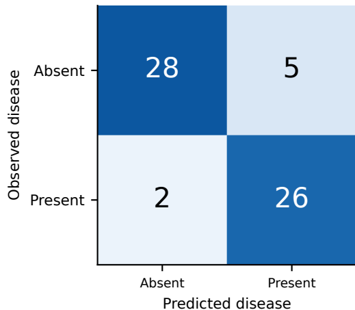
(b) Confusion matrix (n=61)
