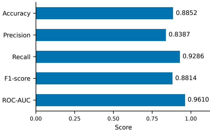
(a) Held-out performance
