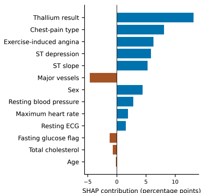
Fig. 6. Original-feature permutation SHAP for one synthetic input. Contributions are in probability percentage points; baseline 41.48% plus all signed contributions gives 83.89%. Positive bars increase the model output; negative bars decrease it. This is not a patient outcome or causal effect.
