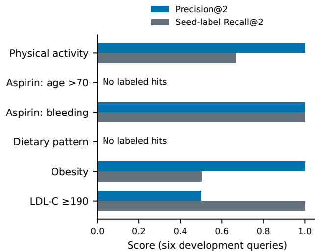
Fig. 4. Retrieval diagnostics for six development queries. Recall uses the stored seed-label set, not exhaustive clinical relevance judgments. Zero-hit topics remain visible.
