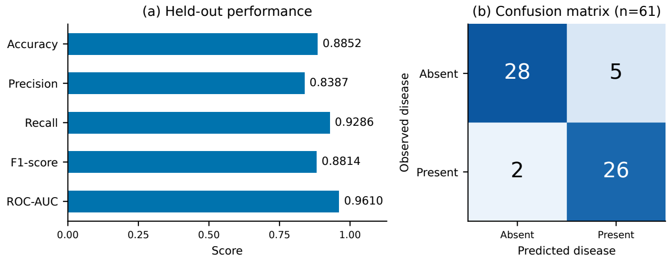
Fig. 3. Selected logistic model on the fixed 61-record holdout. Classification metrics use threshold 0.5; ROC-AUC uses probabilities. The confusion matrix contains raw counts (TN=28, FP=5, FN=2, TP=26).
