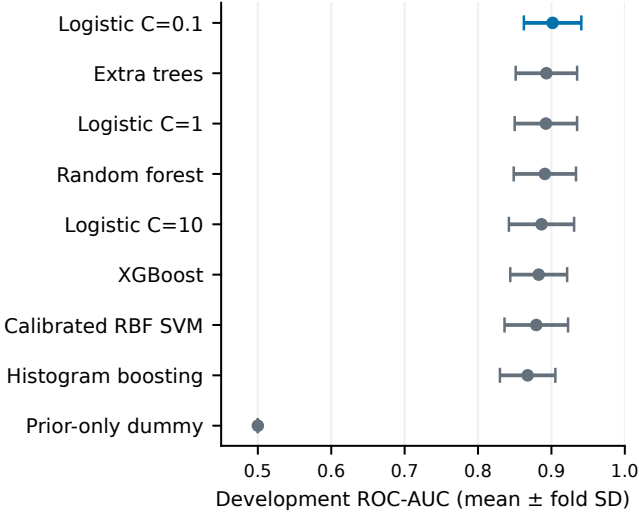
Fig. 2. Development ROC-AUC across nine configurations. Points show means over 15 repeated stratified folds; bars show one fold standard deviation, not confidence intervals. The folds overlap.
