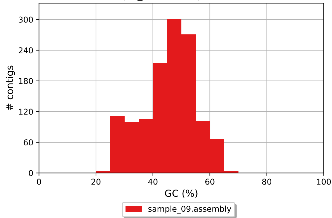
sample_09.assembly GC content
