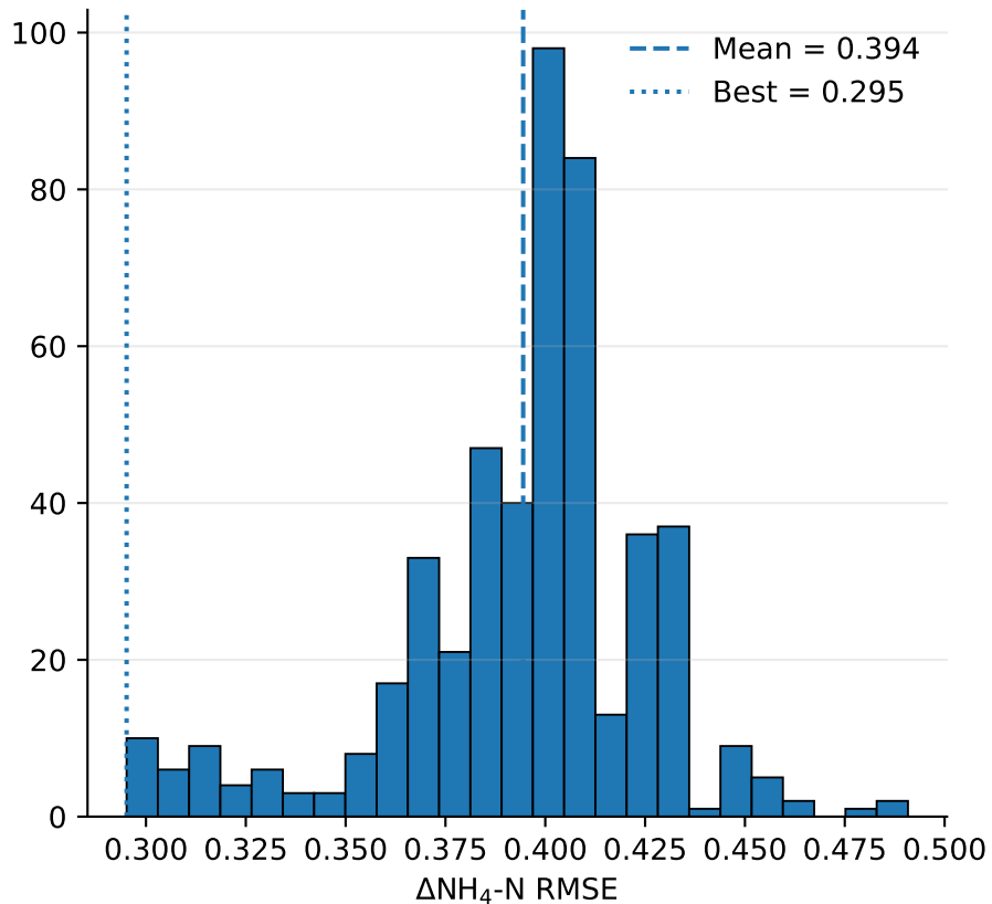
Four-sensor configuration performance: \text{NH}_4\text{-N}
