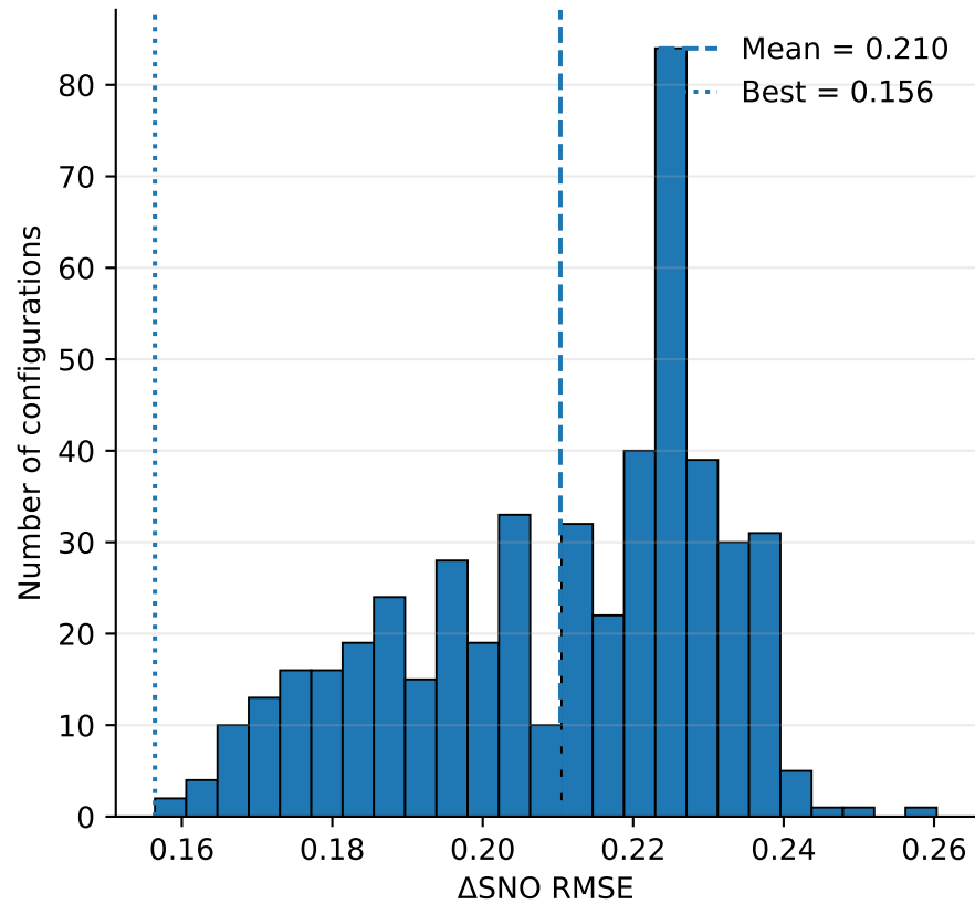
Four-sensor configuration performance: SNO
