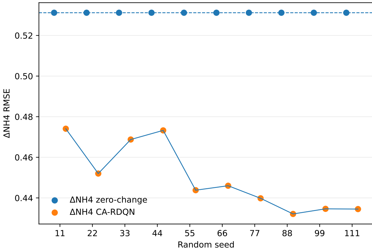
CA-RDQN performance across independent seeds
