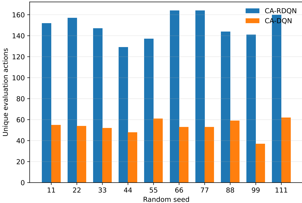
Policy diversity across independent seeds
