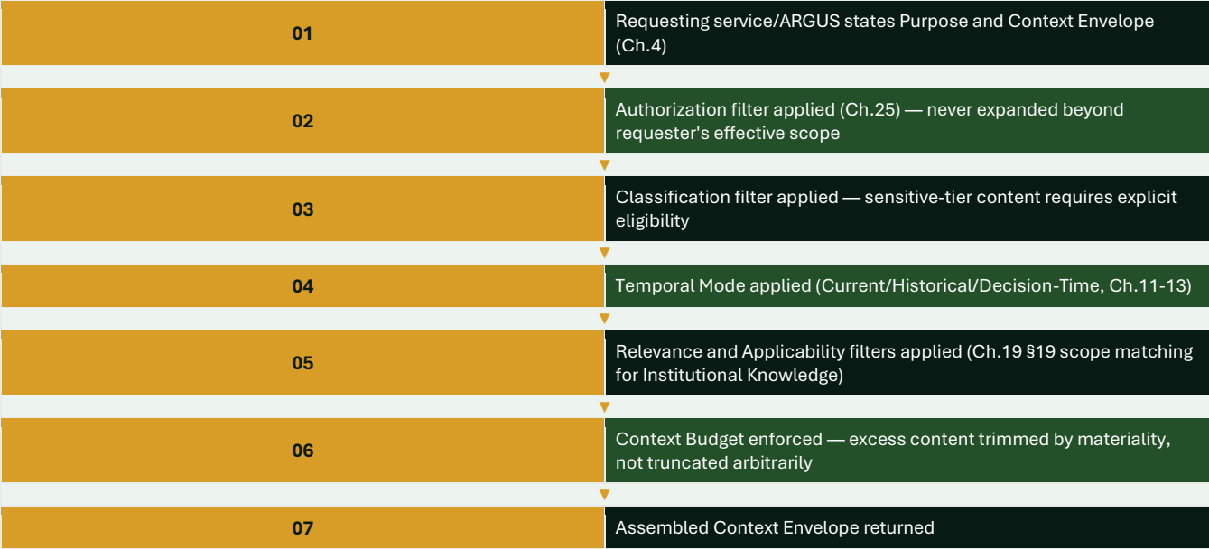
Figure 4. Context Assembly Flow — minimum-necessary retrieval, never a full institutional context dump.
