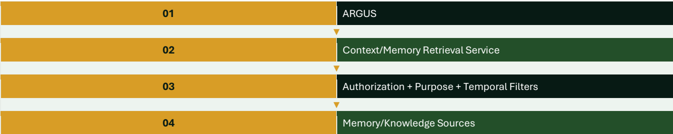
Figure 5. ARGUS's memory access path — no AI-only unrestricted retrieval path exists.
