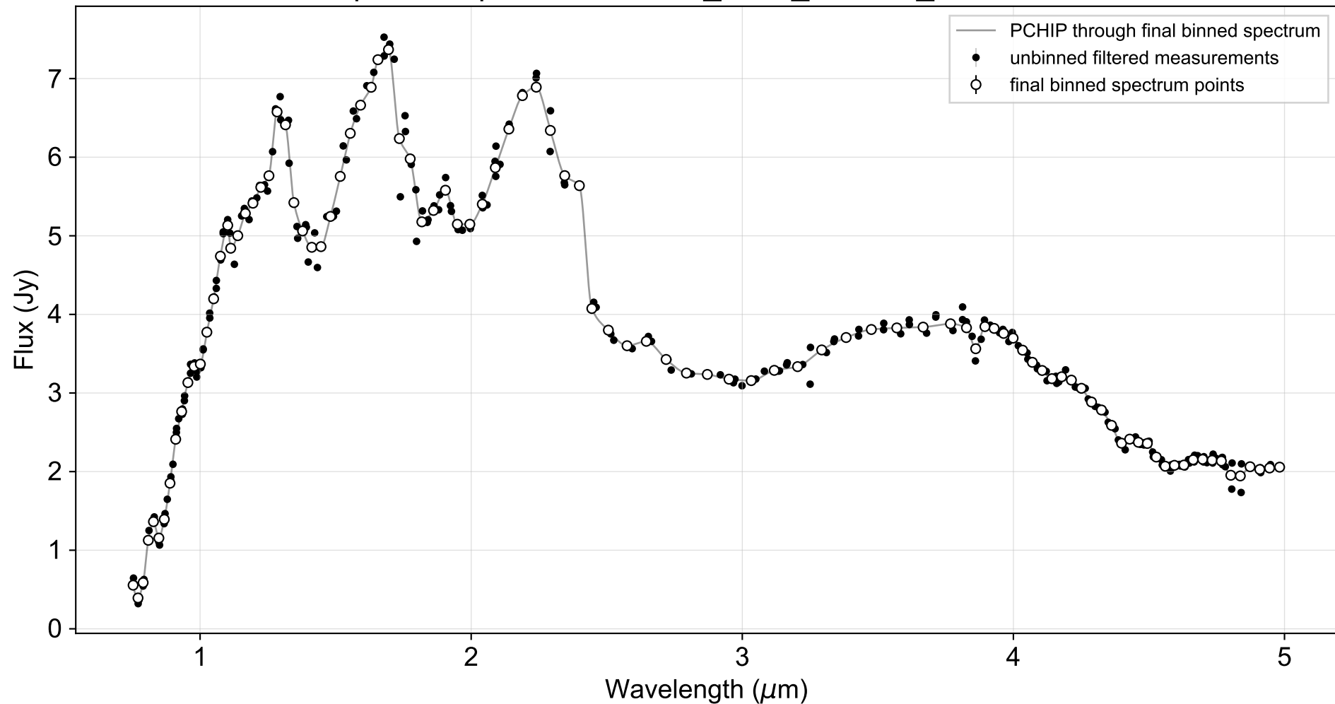
\times 10^{-2} SPHEREx aperture spectrum of UCS_0972_2MASS_J05392474+4038437
