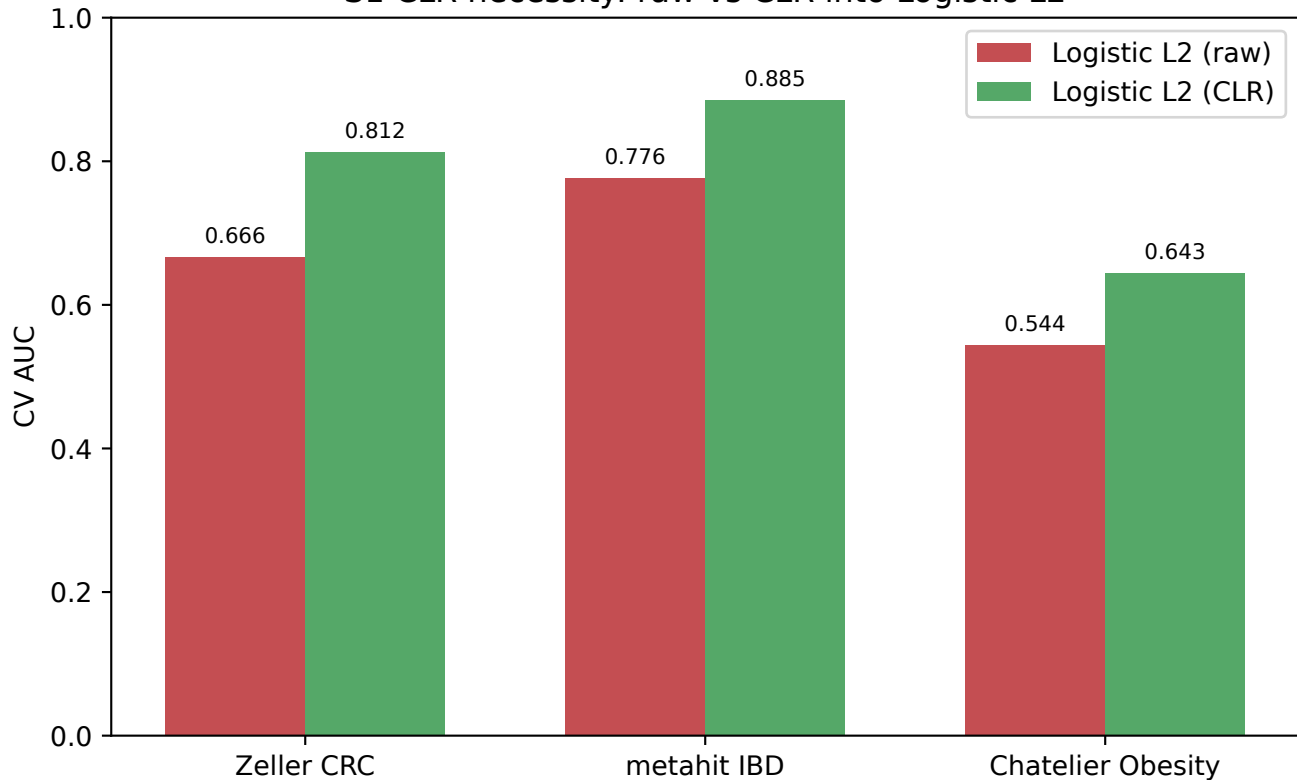
S1 CLR necessity: raw vs CLR into Logistic L2
