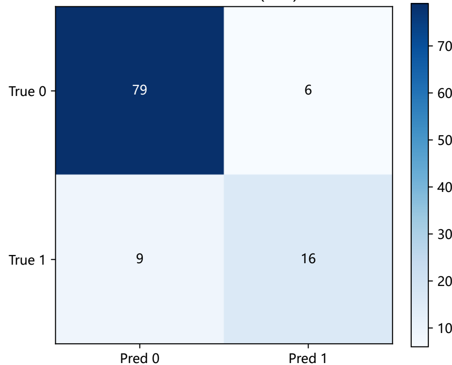
metahit IBD L2(CLR)
