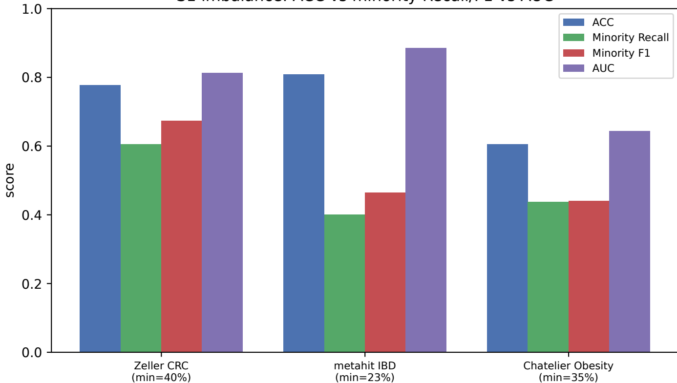
S1 imbalance: ACC vs minority Recall/F1 vs AUC
