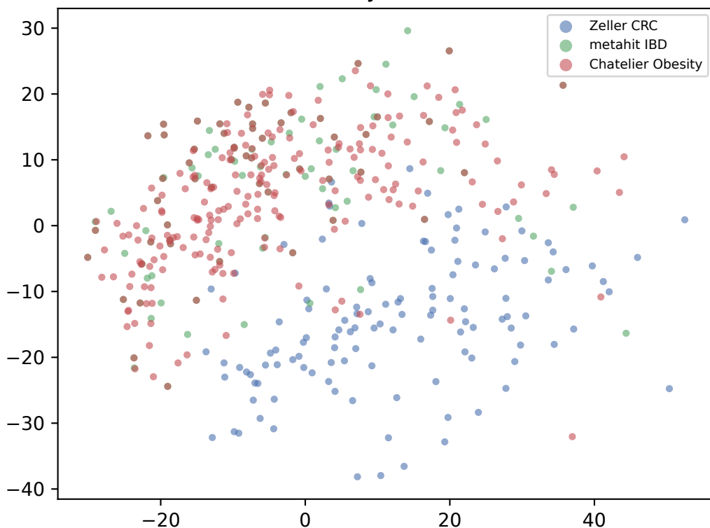
PCA (by disease)
