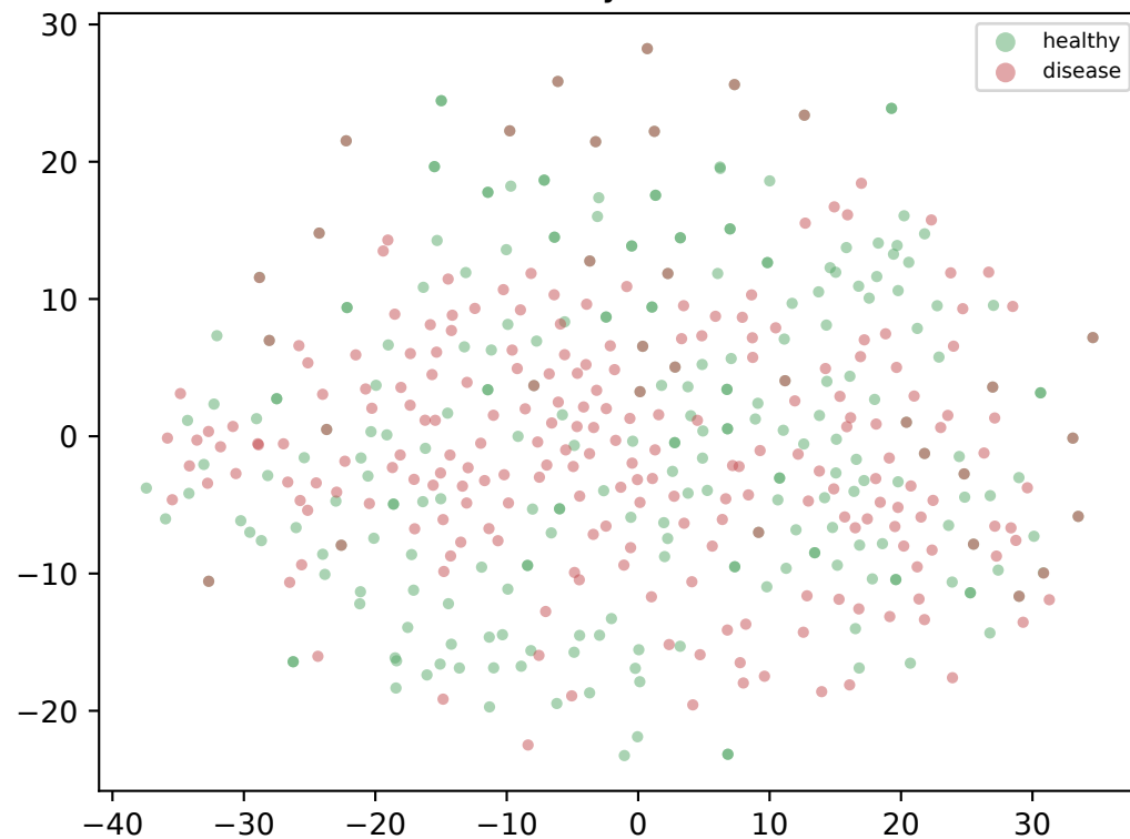
t-SNE (by disease)
