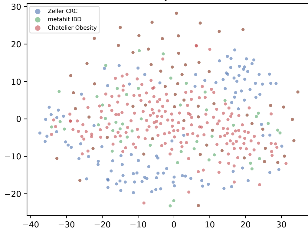
t-SNE (by disease)
