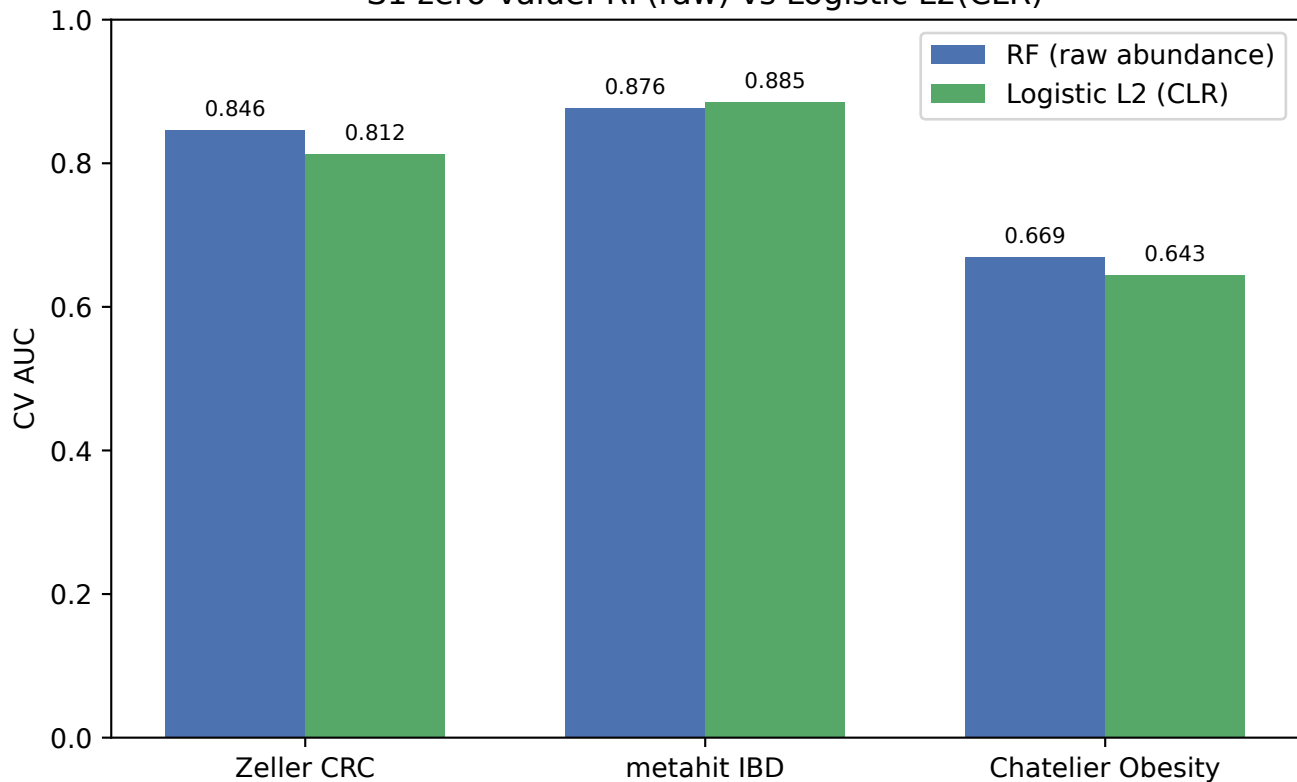
S1 zero-value: RF(raw) vs Logistic L2(CLR)
