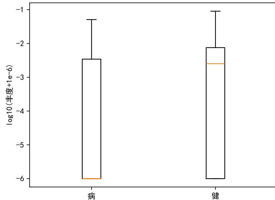
Obesity Top特征 AUC=0.639 s__Ruminococcus_flavefaciens
