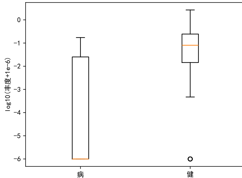
IBD Top特征 AUC=0.815 s__Alistipes_finegoldii
