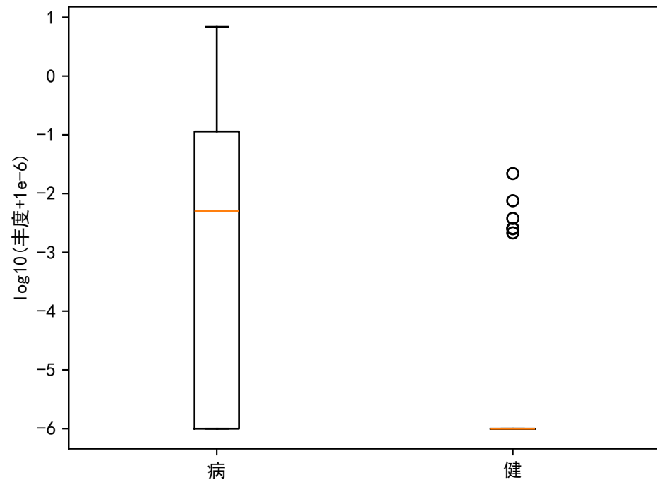
CRC Top特征 AUC=0.758 s__Peptostreptococcus_stomatis
