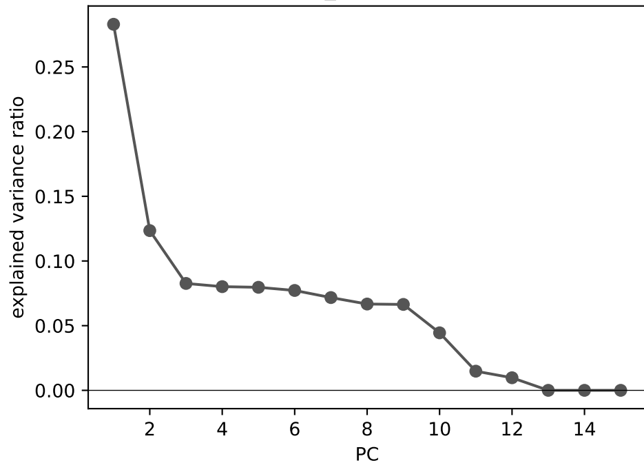
workload_trace PCA scree
