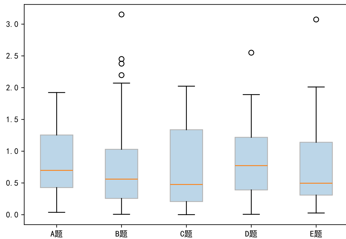
Fairness
