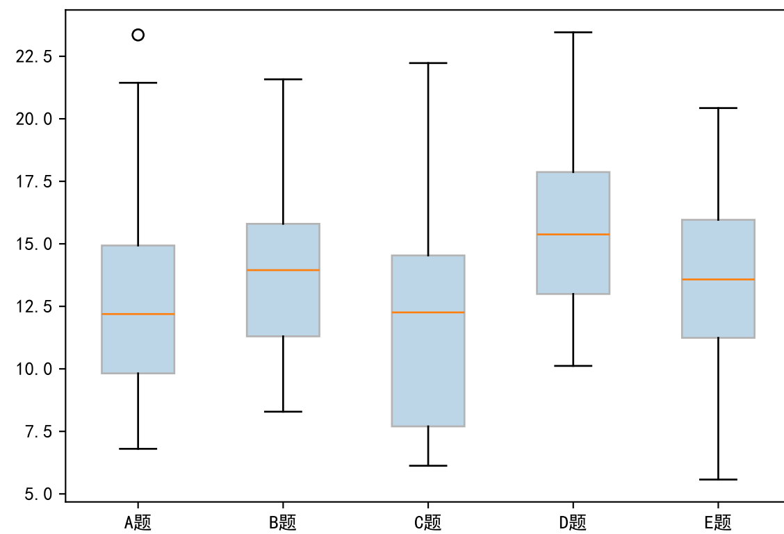
Discrimination
