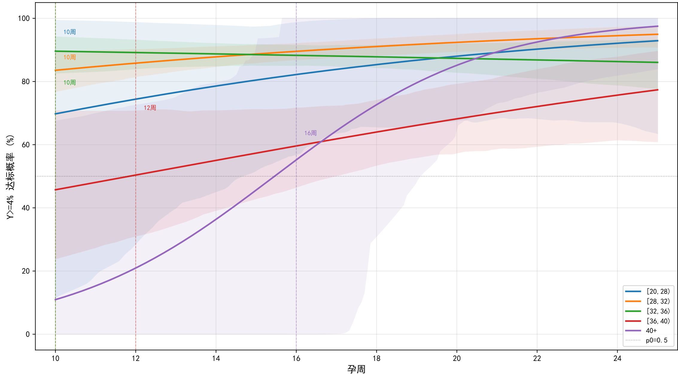
Logistic回归估计的各BMI组达标概率曲线 (95% Bootstrap CI)
