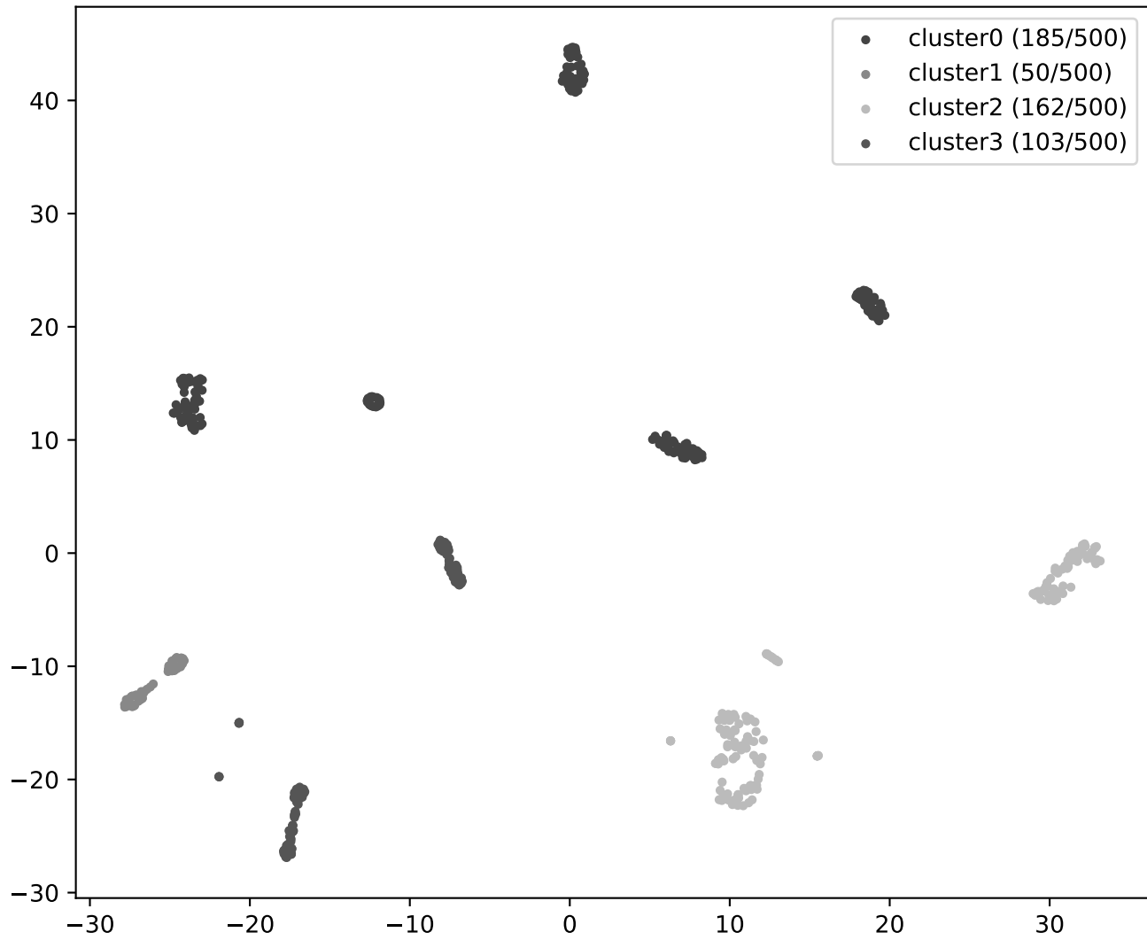
workload_trace task clustering t-SNE (k=4)
