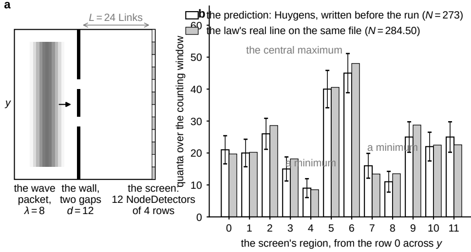
Fig. 2 The two slits, the one computed file (computed; the run's N a run; clicks). (a) Universe24 as its file declares it. The flat lattice has 45 \times 48 Nodes. The wave packet of light, at the wavelength 8 Links, is laid over the columns 4 to 16 (the grey raised cosine) and moves along +x . The wall at the column 20 has two gaps of three rows, 12 Links apart. The screen at the column 44, 24 Links from the wall, is twelve declared NodeDetectors of four rows each. (b) The screen's row per region over the counting window of the intervals 45 to 130. The design's blind row, the law's line in real arithmetic at the design's initial data (the Huygens sum of the archived file's comment, one computation under two names), written before the run, is hollow ( N = 273 , its bars summing to 275 by the per-Node rounding, with the draw's scatter \sqrt{NP(1-P)} per region). Beside it, in grey, is the law's real line stepped on the same file at the initial data as the commit holds them ( N = 284.50 in the implementation's labels, 284.7 in the physical ones). The run gives N = 285 at both seeds. The points are the seed-24 clicks per region of the one run, from the archived row the draw's gate holds (computed, a run); the run a check, no run made for the drawing
